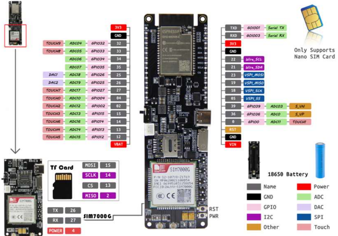
ESP32 SIM Card T-SIM7000G V1.1
